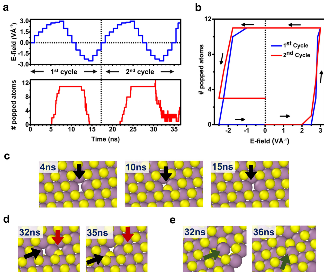
Fig. 2 Bipolar switching characteristics of monolayer MoS 2 comprising of 12 S monovacancies in one plane. a Plot of applied electric field and no. of popped atoms vs. simulation time. b Hysteresis plot showing the change in popped atom count with the applied field. The order of application of the field is 0→3→0→−2.5→0. Atomistic snapshots zooming-in at the vacancy locations at different points of time displaying various events, c initial vacancy location (4 ns), S atom popping after set (10 ns), popped atom returning after reset (15 ns), d secondary popping (32 ns) during reset and its recovery (35 ns) with the positive field of 2 VÅ −1 in next cycle, and e localized distortion during reset (32 ns) and its recovery (36 ns). Black, red, and green arrows highlight the vacancy locations, secondary popped atoms, and distorted locations.
