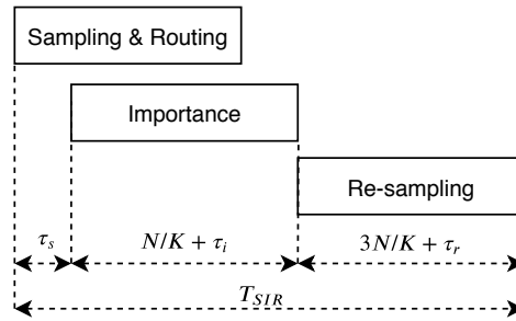
FIGURE 9: Timing diagram for SIR operations of the proposed design.
