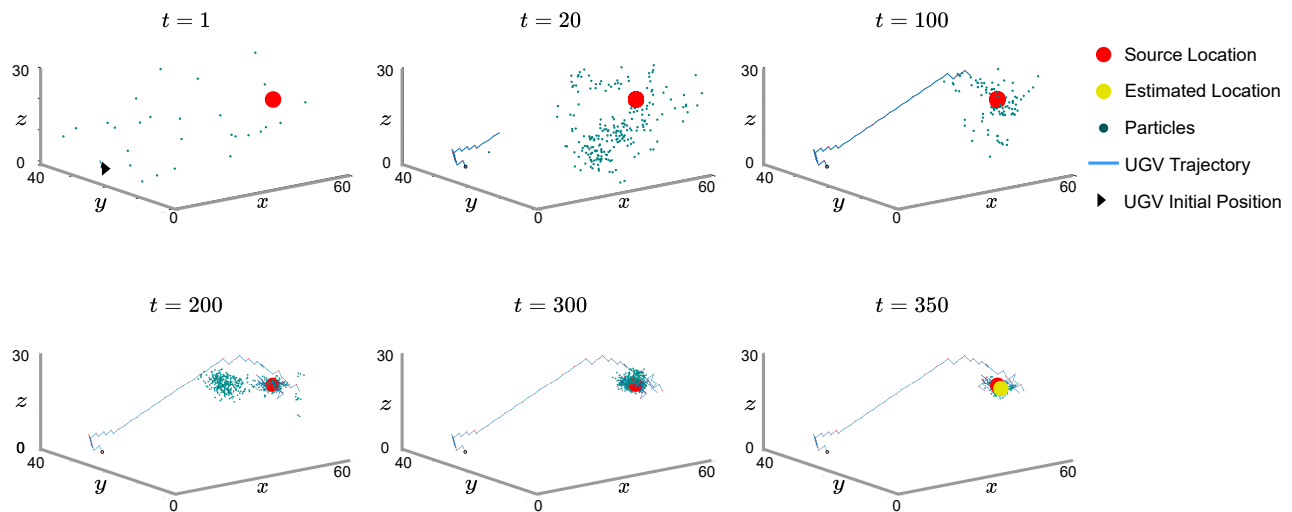
FIGURE 13: 3D source localization experimental result. The source is positioned at [40, 5, 25] , and the initial position of the UGV is [10, 30, 0] . The model is run over 350 time-steps for 512 particles. Here, the UAV traverses in three dimensions to move towards the source. The error between the source and the estimated location is 0.83. The probabilities \alpha and \beta are set as 0.8 and 0.4, respectively. [Figure updated]
